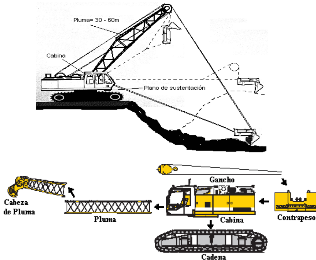
FIGURA 5-2: Partes Dragalina
